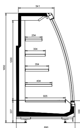
NordicStar SV5 30-89-165
