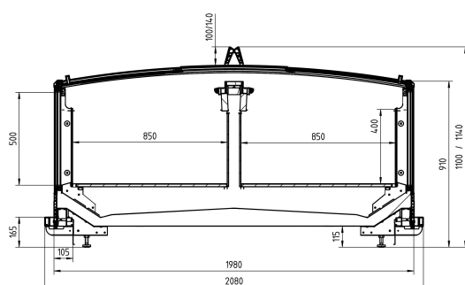
IS7-200-90-250-F-cross-section-curved-lids-115mm copia
